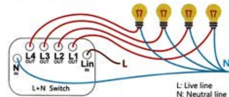
Diagram 1: For Switches With Neutral (L+N Switch)
