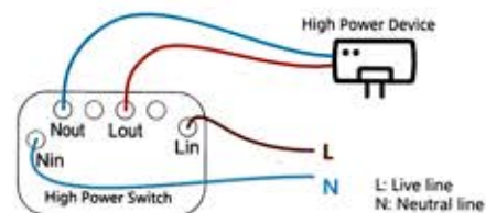
Diagram 2: For 30A/20A High Power Switches
